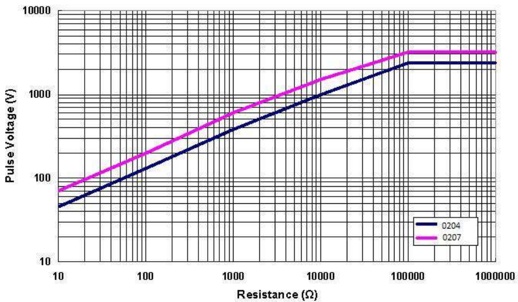
10/700µs Lightning Surge
